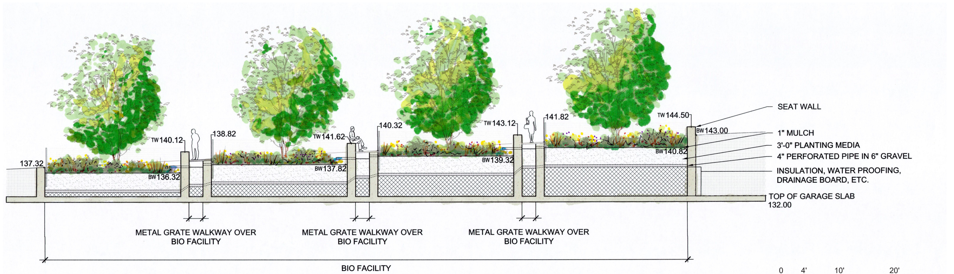
4TH ST, NE BIORETENTION SECTION A-A'
